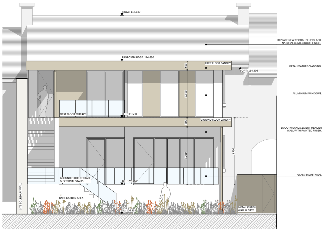
Rear Elevation 1:100
