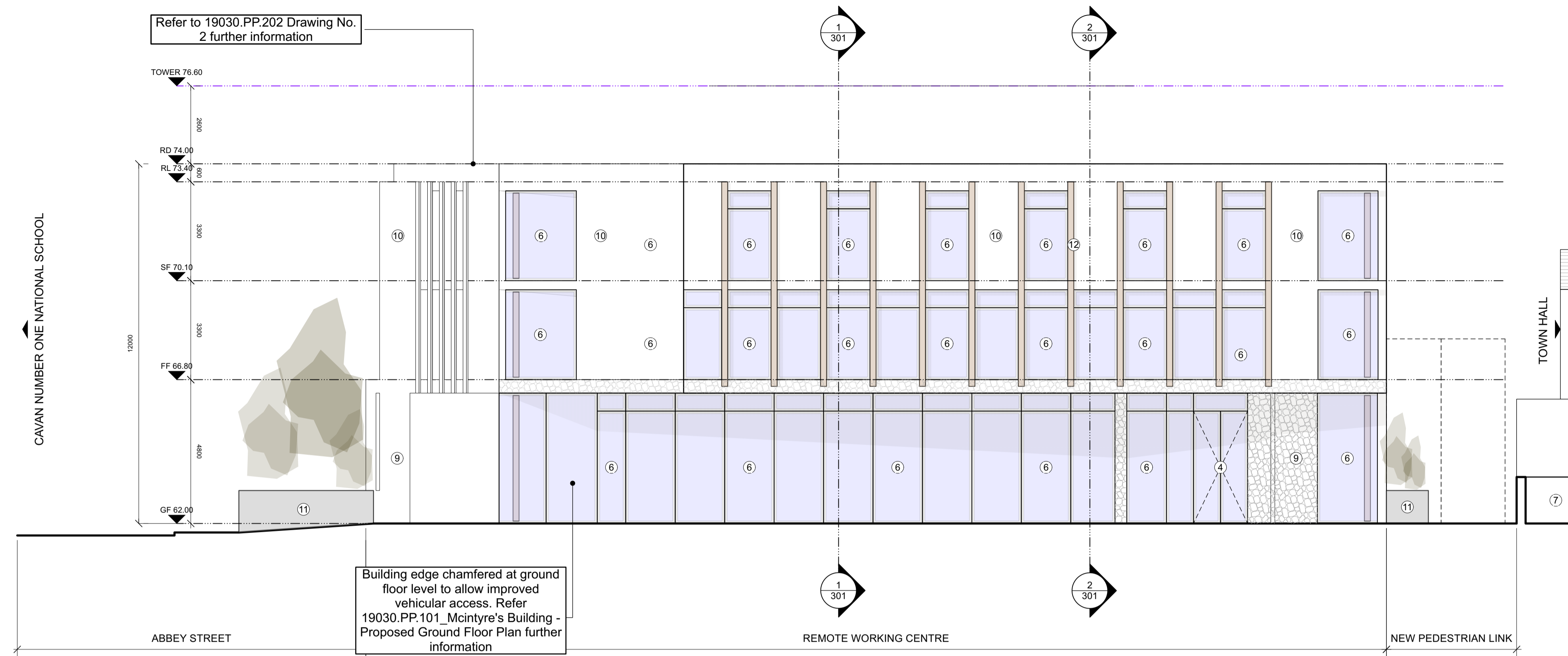
1 Proposed Elevation 1 PP.201 Scale: 1:100
