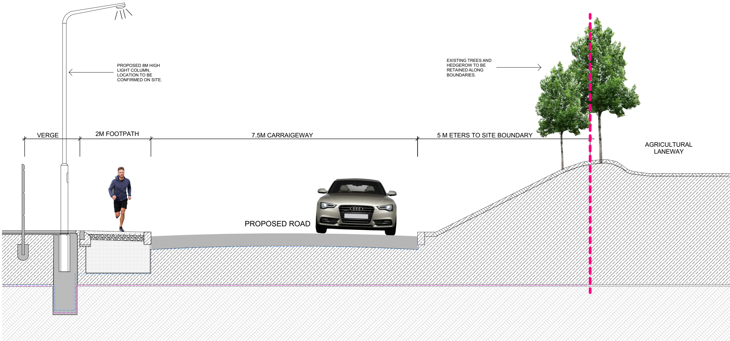
Road Section A-A
