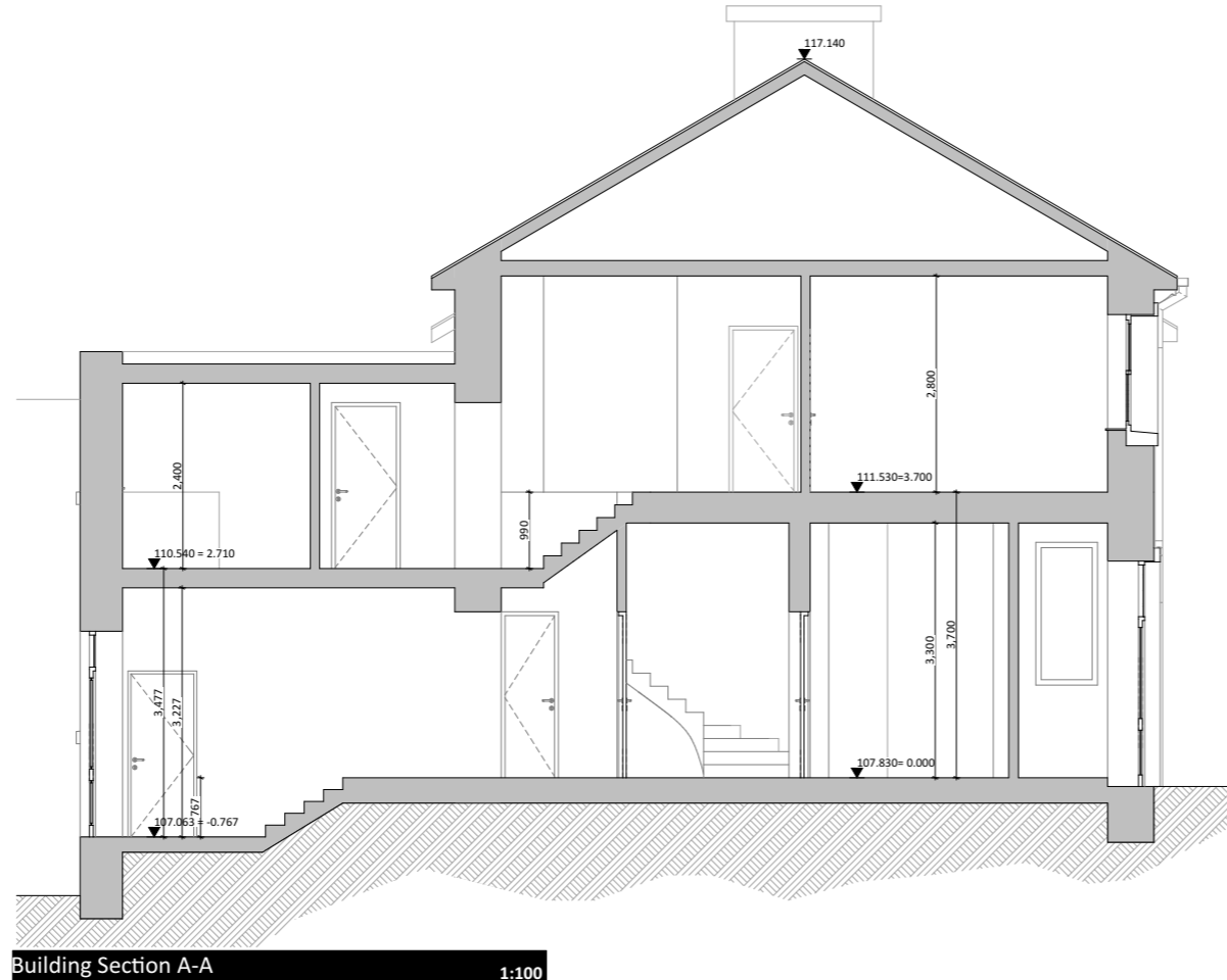
Building Section A-A 1:100
