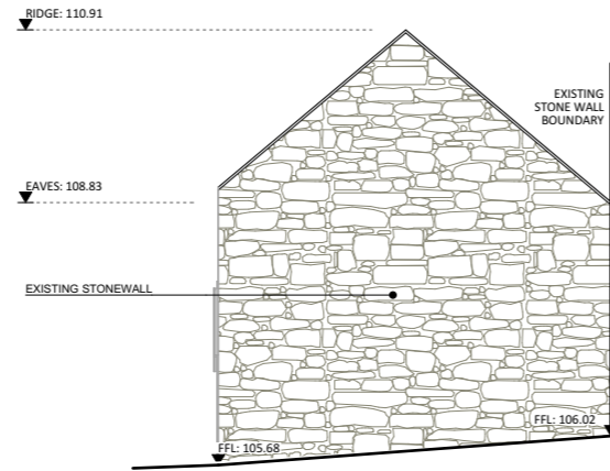
Shed - Rear Elevation 1:100
