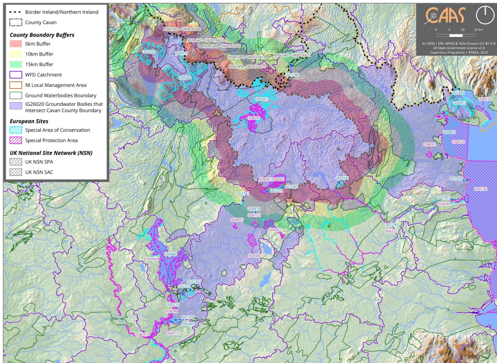
Figure 3.3 Groundwater sensitive European sites that share groundwater bodies with County Cavan 17
