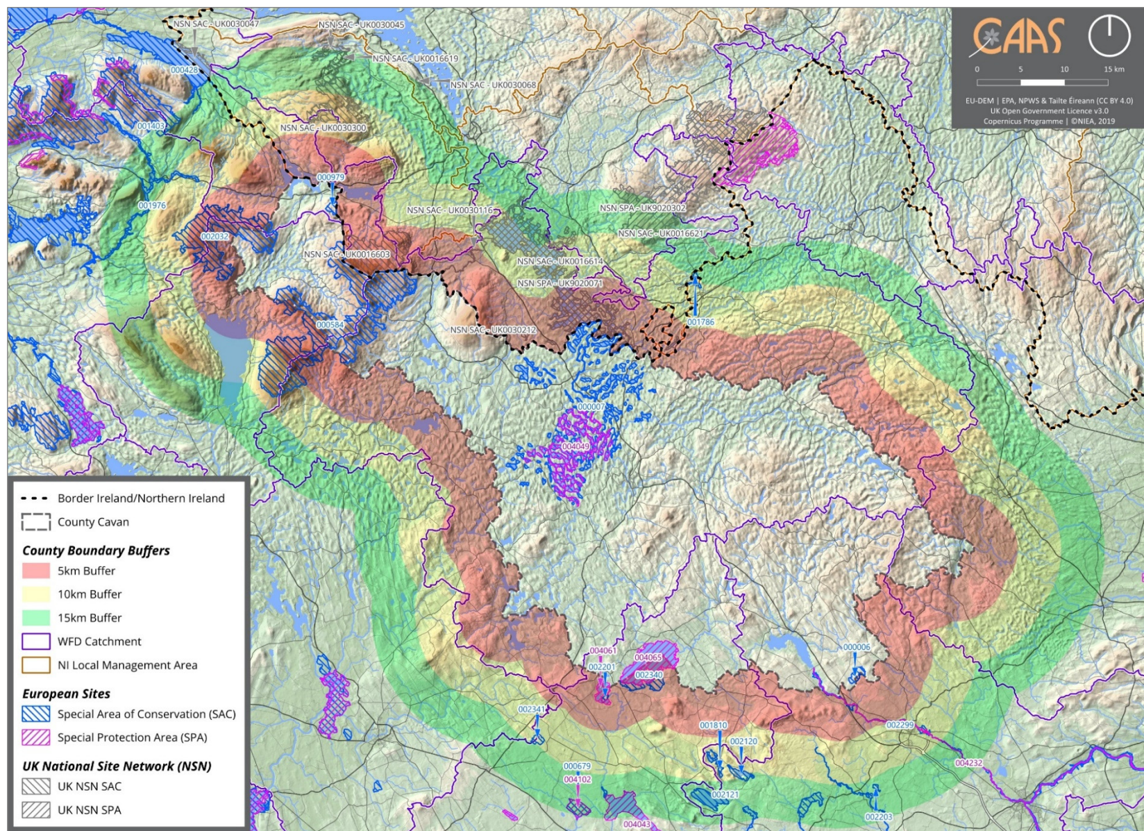
Figure 3.1 European sites within a 15 km buffer zone of the area to which the Proposed Variation relates 15
