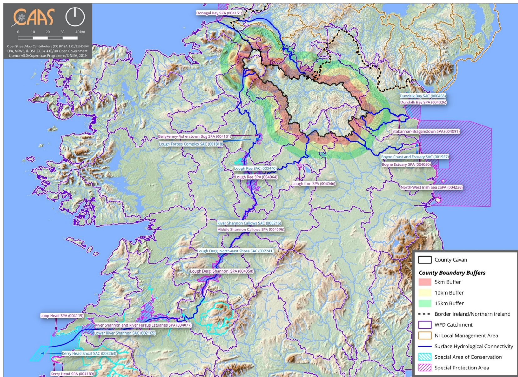
Figure 3.2 European sites with surface hydrological connectivity to County Cavan 16
